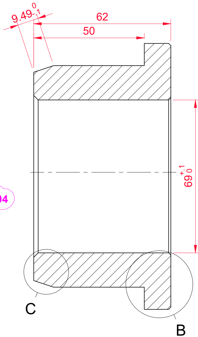
SECTION A-A (1:1)
