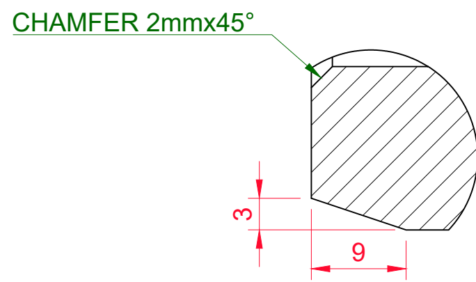
DETAIL C (2:1)
