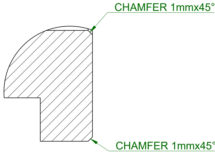
DETAIL B (2:1)
