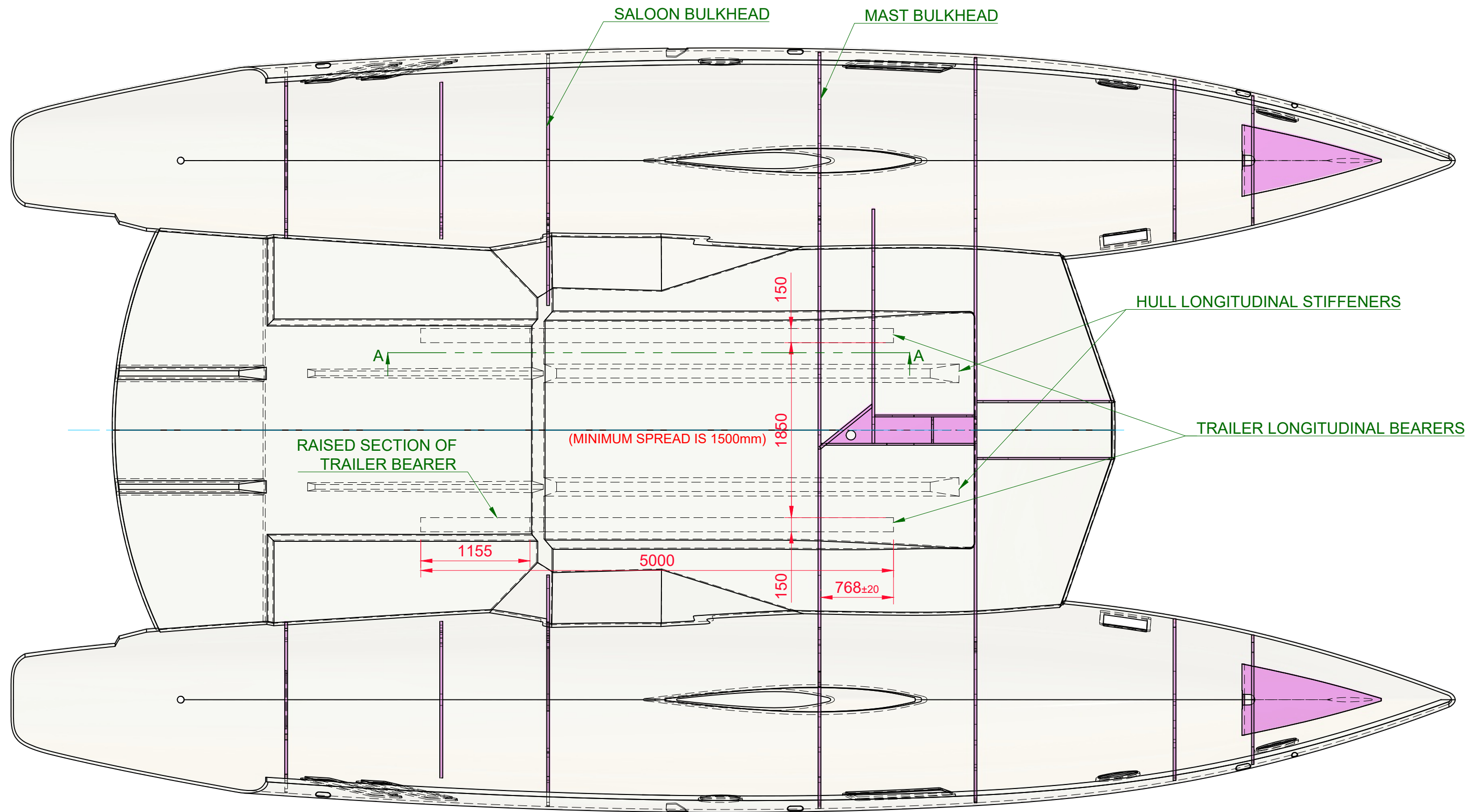
PLAN VIEW OF K500SE HULL, BULKHEADS, & TRAILER BEARERS BELOW
